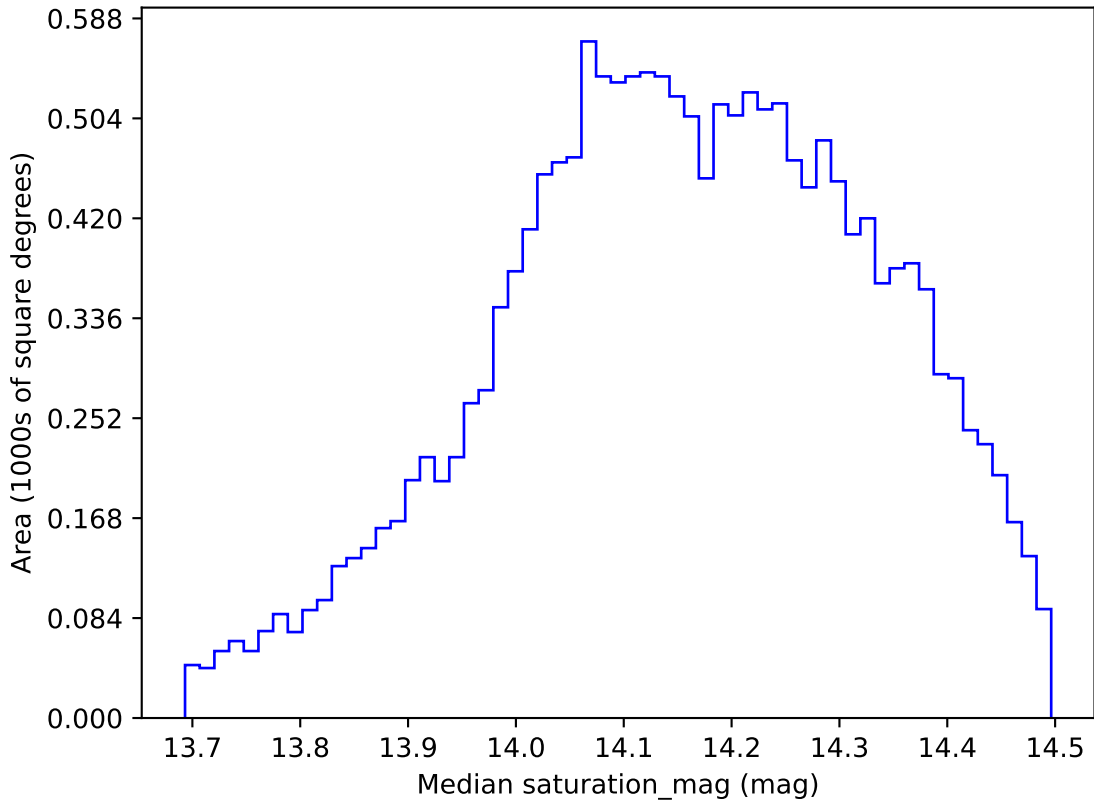
too_elab_r8_d2_griz_v3.4_10yrs WFD all bands: Median saturation_mag
