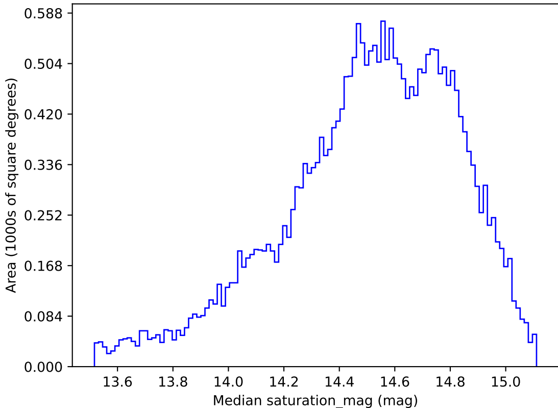
too_elab_r8_d2_griz_v3.4_10yrs All sky g band: Median saturation_mag
