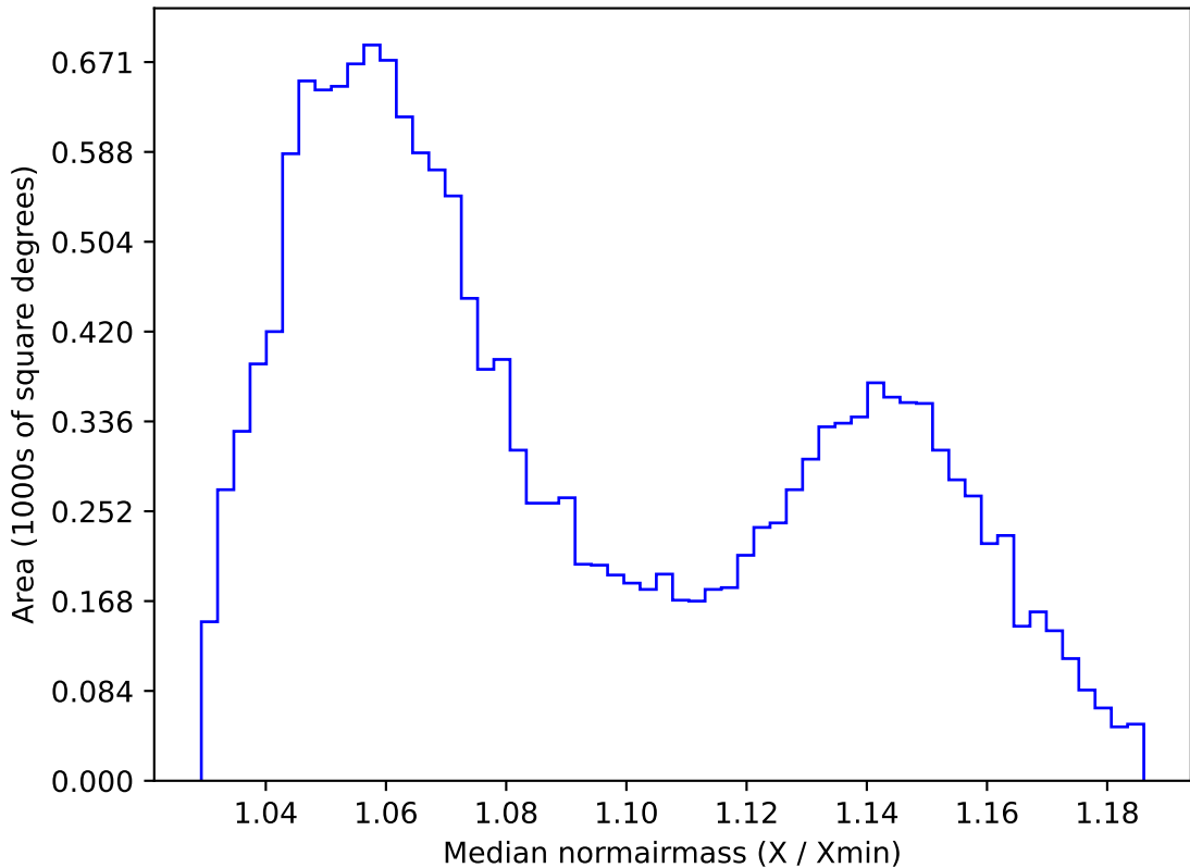
too_elab_r8_d2_griz_v3.4_10yrs WFD y band: Median normairmass
