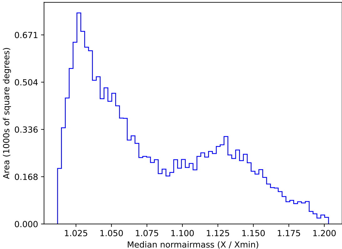
too_elab_r8_d2_griz_v3.4_10yrs WFD u band: Median normairmass
