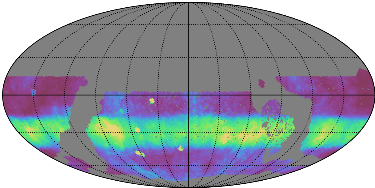
too_elab_r8_d2_griz_v3.4_10yrs WFD r band: Median normairmass
