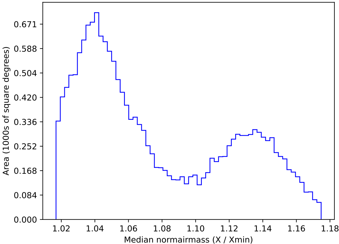
too_elab_r8_d2_griz_v3.4_10yrs WFD i band: Median normairmass
