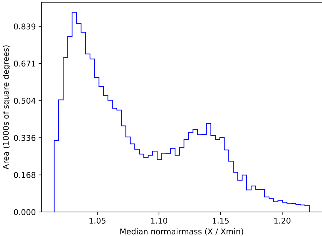
too_elab_r8_d2_griz_v3.4_10yrs WFD g band: Median normairmass
