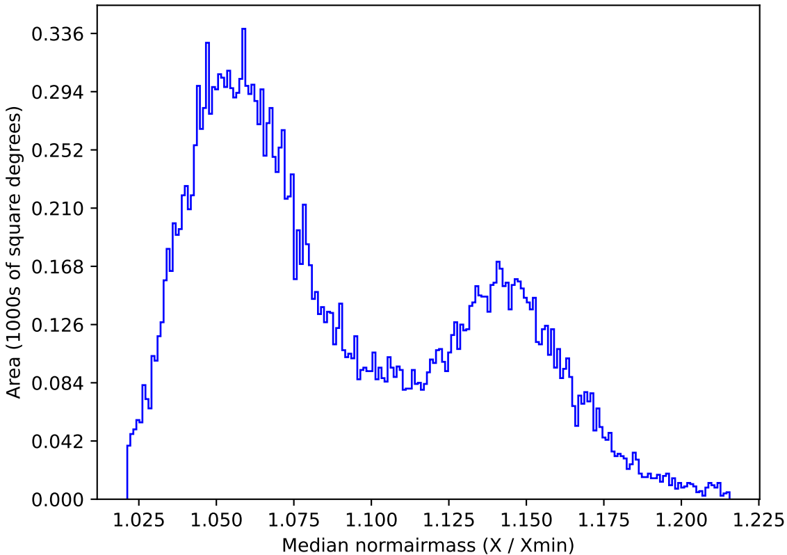
too_elab_r8_d2_griz_v3.4_10yrs All sky y band: Median normairmass
