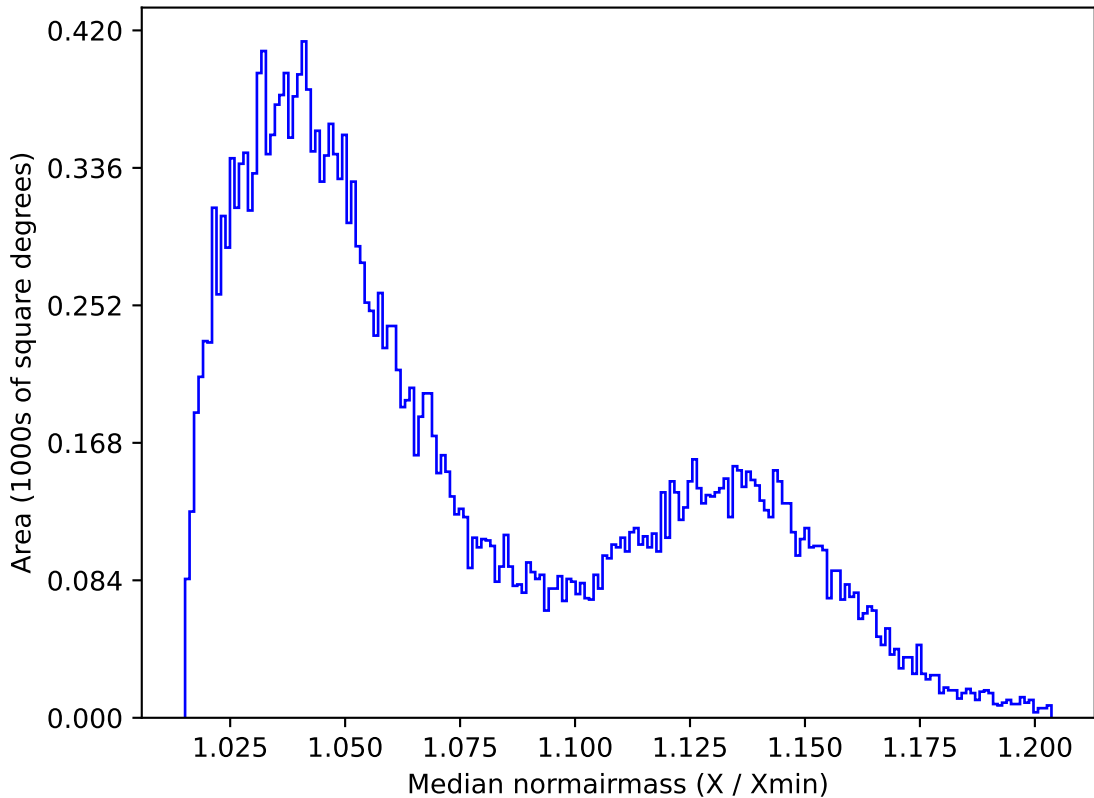
too_elab_r8_d2_griz_v3.4_10yrs All sky i band: Median normairmass
