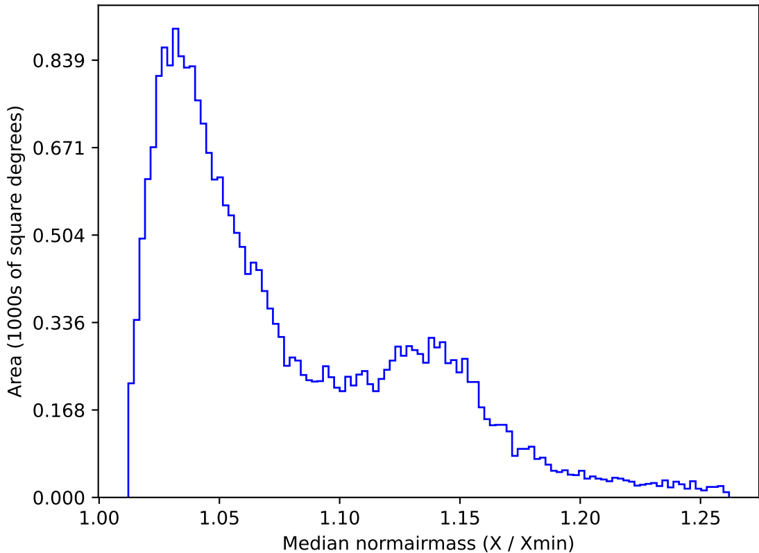
too_elab_r8_d2_griz_v3.4_10yrs All sky g band: Median normairmass
