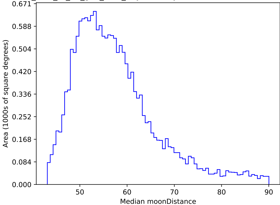
too_elab_r8_d2_griz_v3.4_10yrs WFD y band: Median moonDistance
