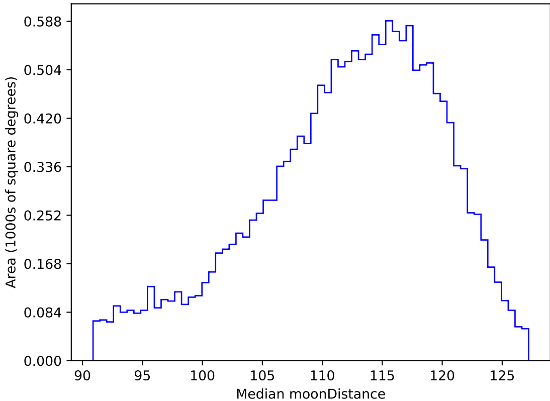
too_elab_r8_d2_griz_v3.4_10yrs WFD r band: Median moonDistance
