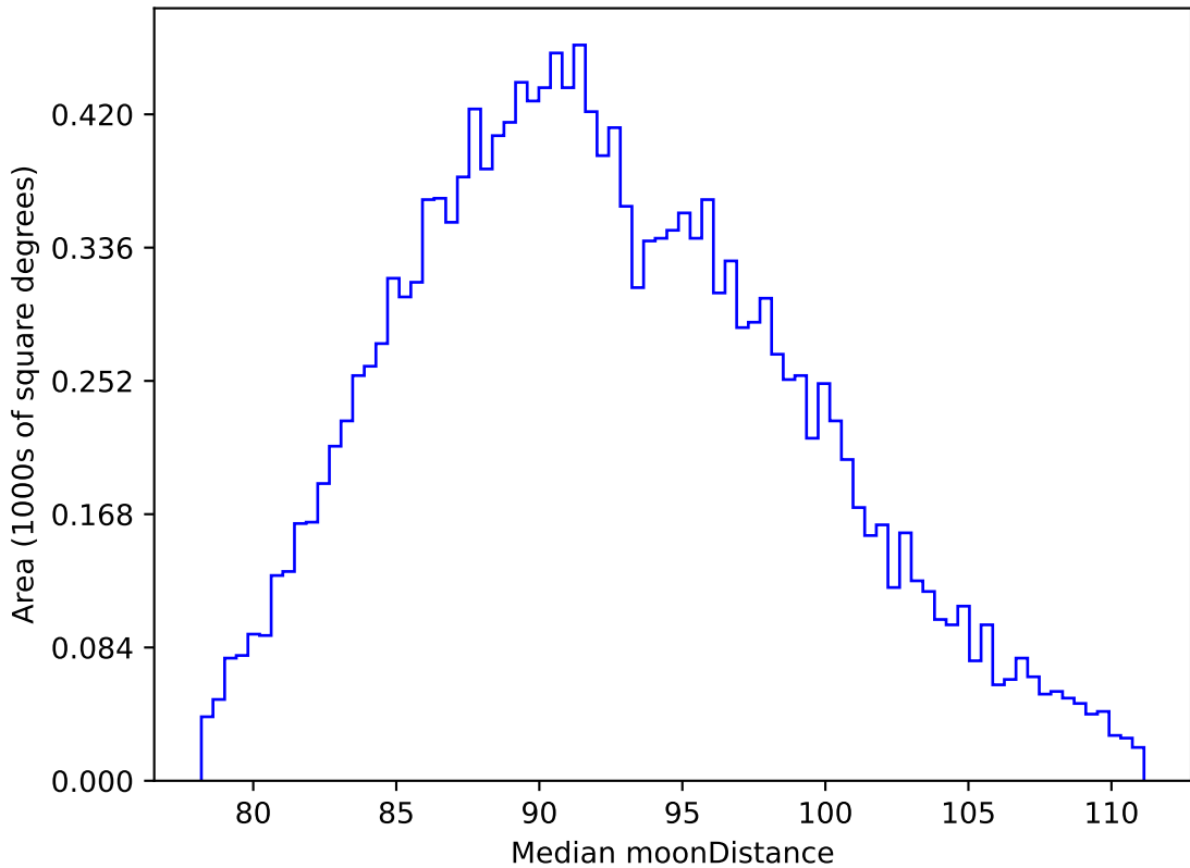
too_elab_r8_d2_griz_v3.4_10yrs WFD i band: Median moonDistance
