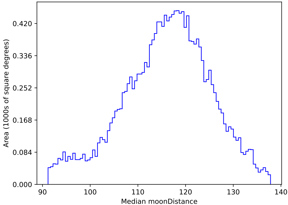
too_elab_r8_d2_griz_v3.4_10yrs WFD g band: Median moonDistance
