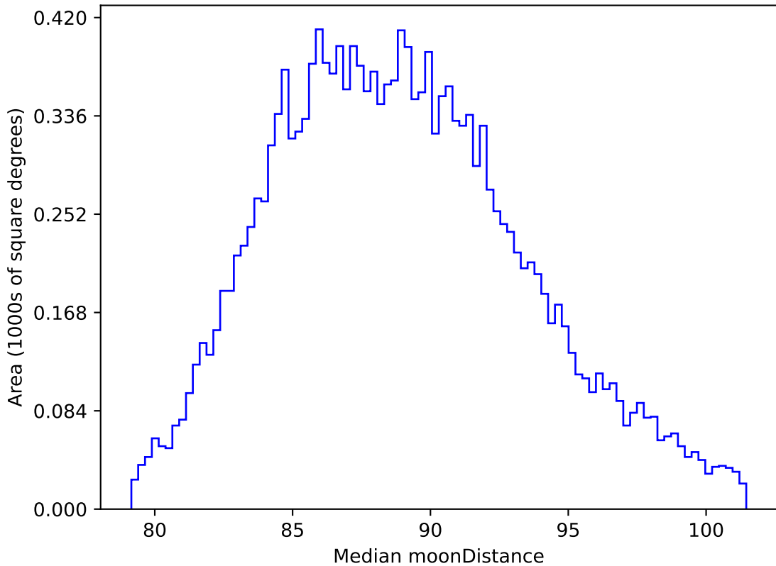
too_elab_r8_d2_griz_v3.4_10yrs WFD all bands: Median moonDistance
