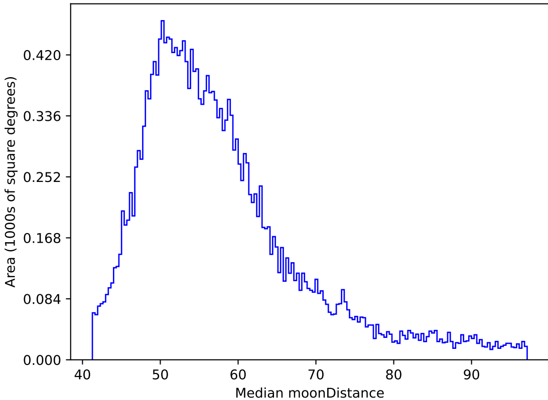
too_elab_r8_d2_griz_v3.4_10yrs All sky y band: Median moonDistance
