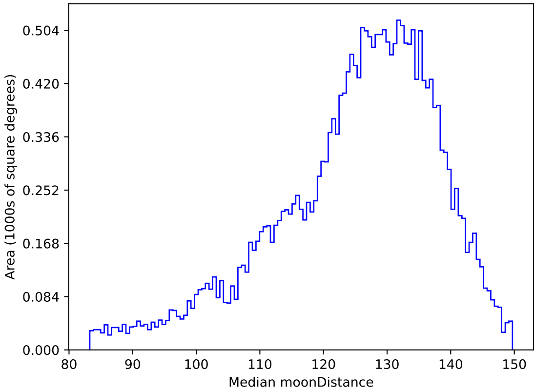
too_elab_r8_d2_griz_v3.4_10yrs All sky u band: Median moonDistance
