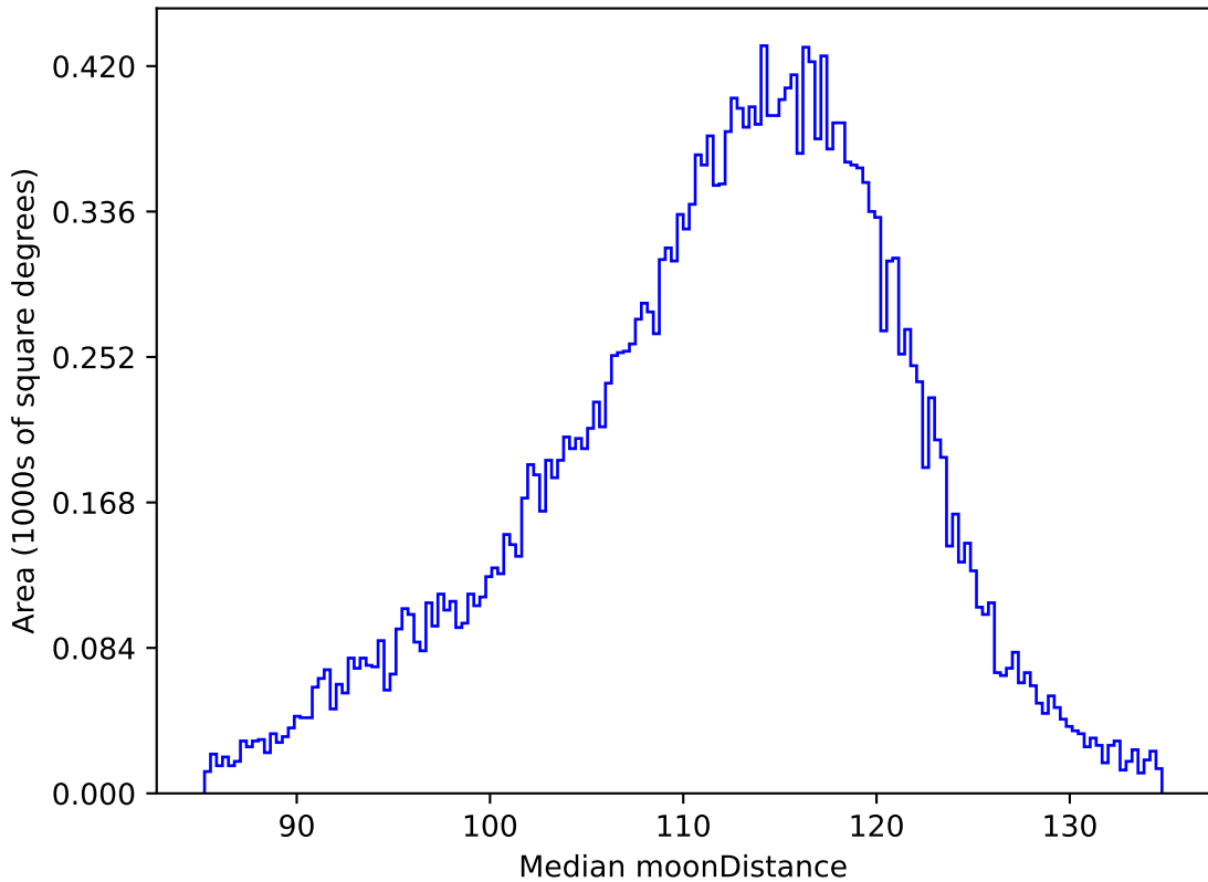
too_elab_r8_d2_griz_v3.4_10yrs All sky r band: Median moonDistance
