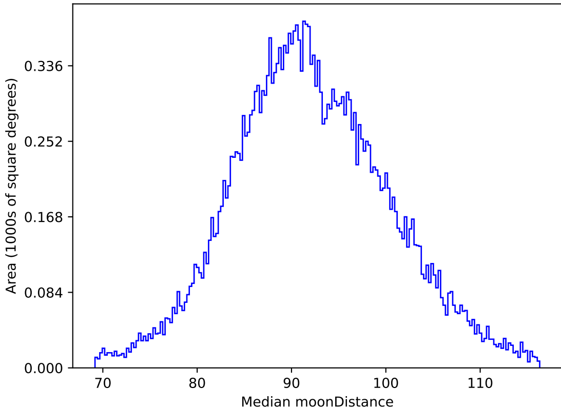
too_elab_r8_d2_griz_v3.4_10yrs All sky i band: Median moonDistance
