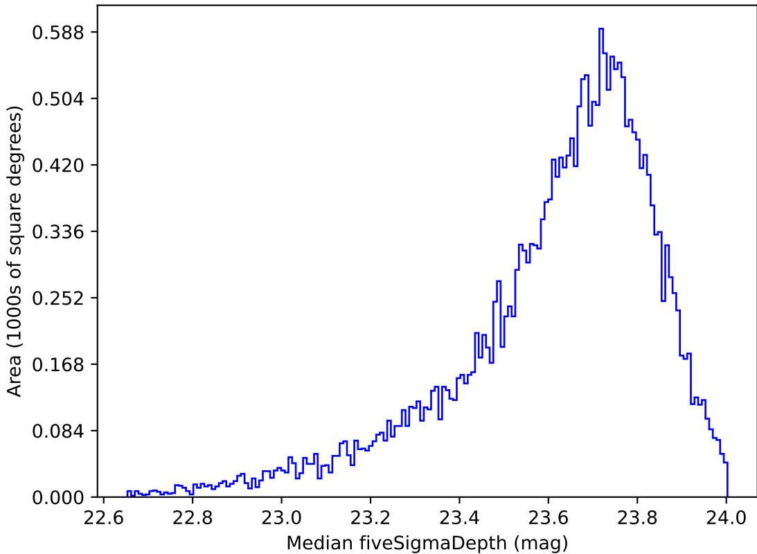
too_elab_r8_d2_griz_v3.4_10yrs Yr 1 i band: Median fiveSigmaDepth
