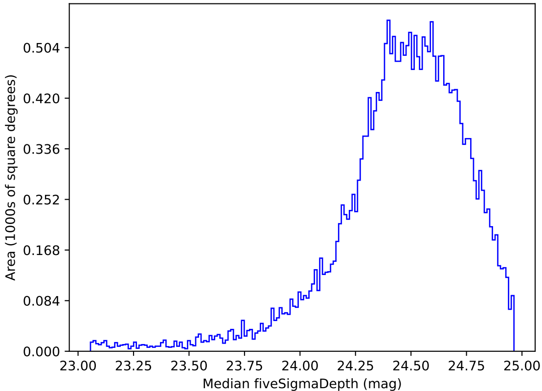
too_elab_r8_d2_griz_v3.4_10yrs Yr 1 g band: Median fiveSigmaDepth
