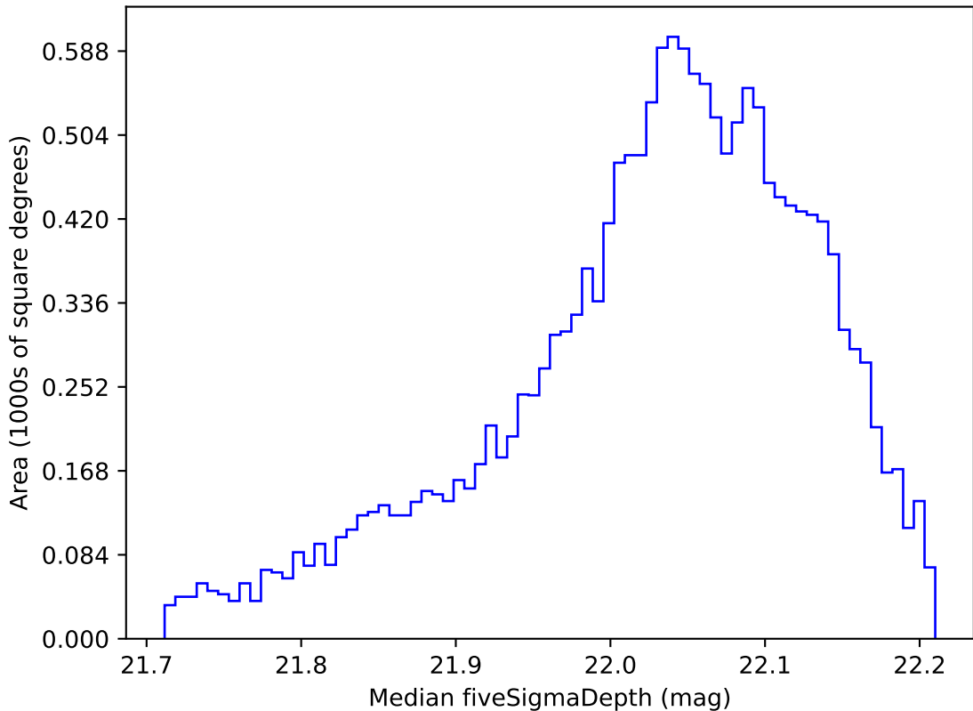
too_elab_r8_d2_griz_v3.4_10yrs WFD y band: Median fiveSigmaDepth
