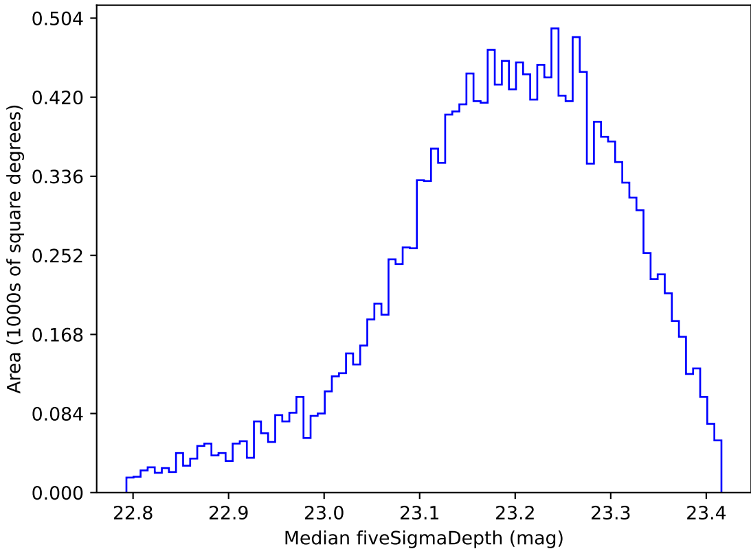
too_elab_r8_d2_griz_v3.4_10yrs WFD u band: Median fiveSigmaDepth
