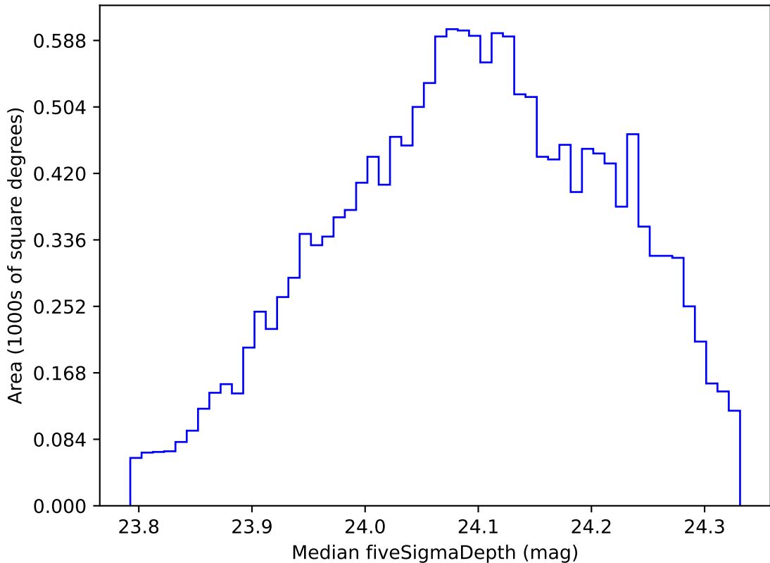
too_elab_r8_d2_griz_v3.4_10yrs WFD r band: Median fiveSigmaDepth
