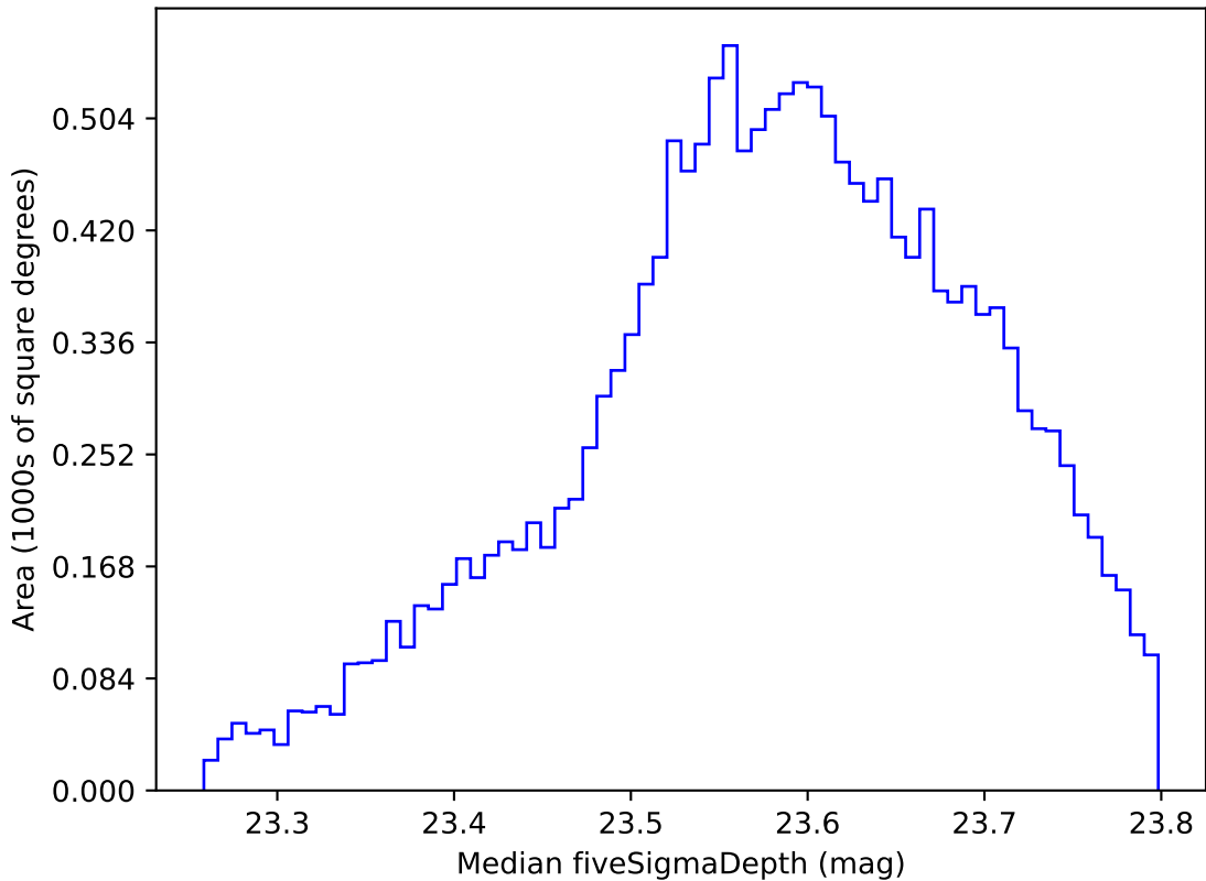
too_elab_r8_d2_griz_v3.4_10yrs WFD i band: Median fiveSigmaDepth
