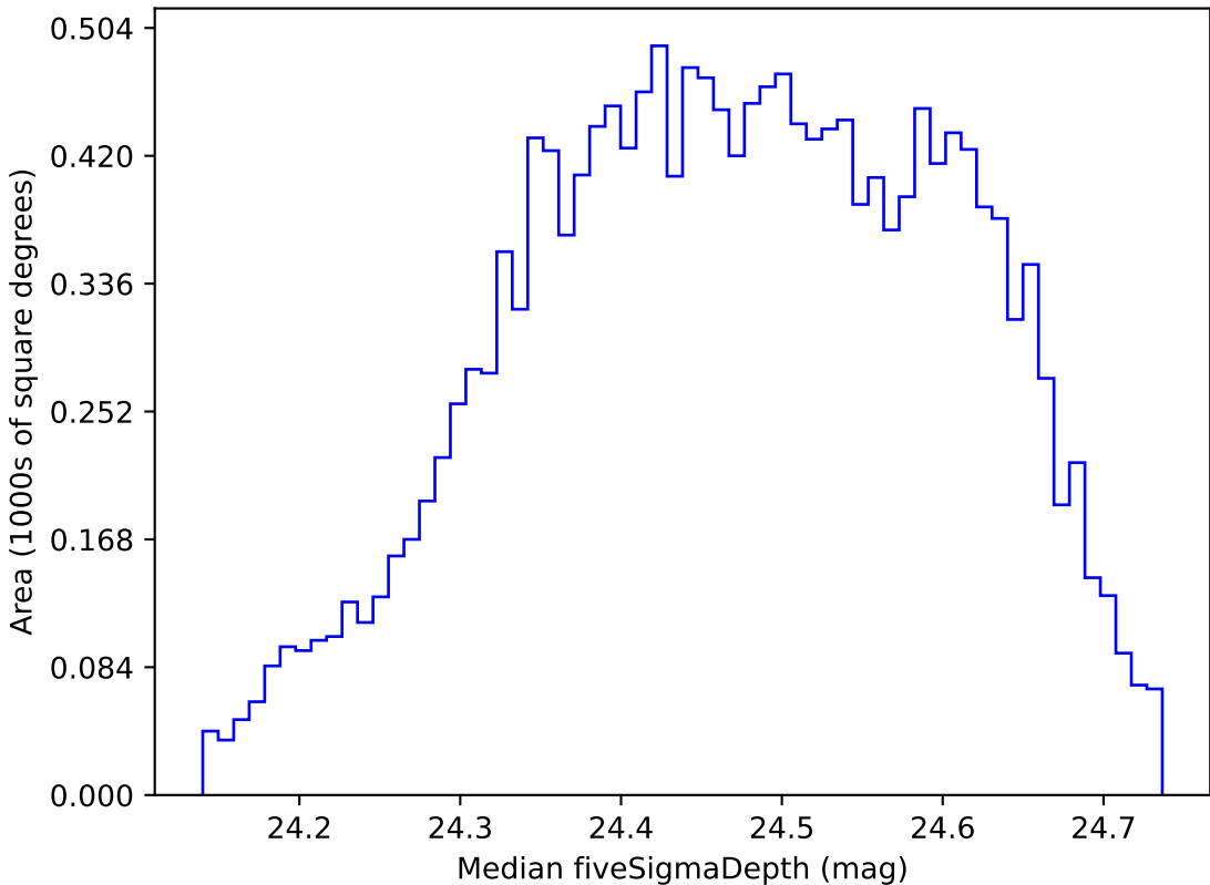
too_elab_r8_d2_griz_v3.4_10yrs WFD g band: Median fiveSigmaDepth
