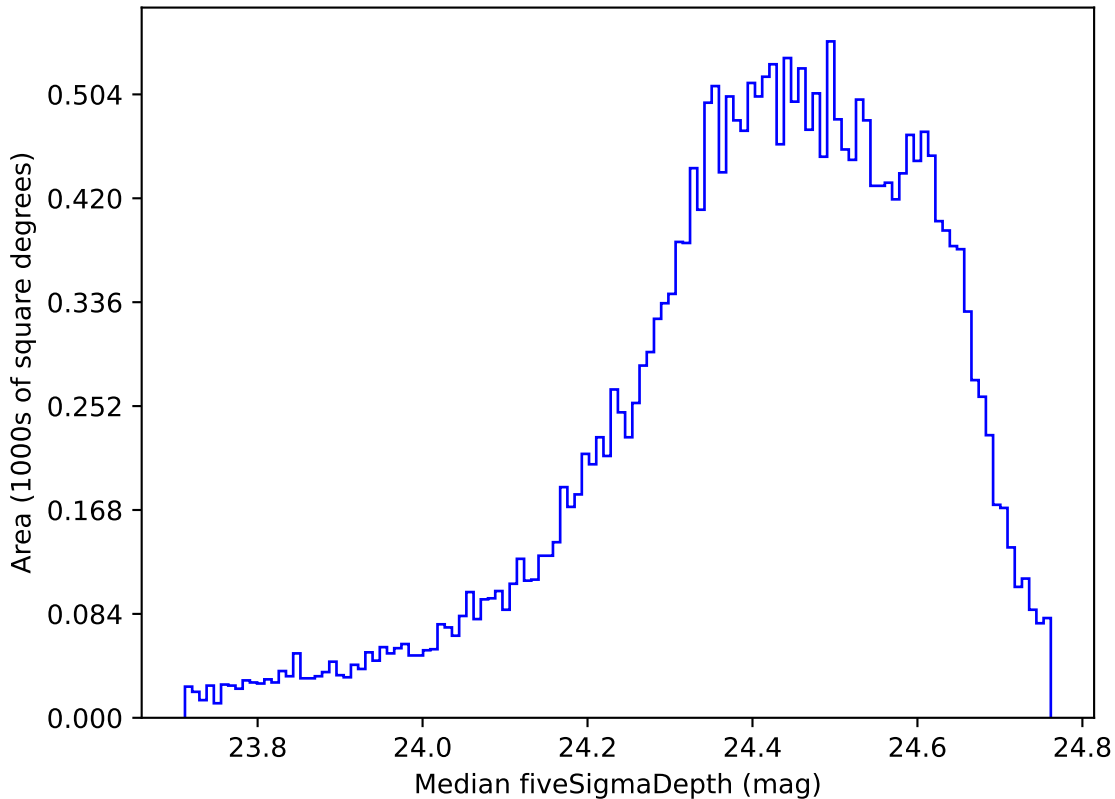
too_elab_r8_d2_griz_v3.4_10yrs All sky g band: Median fiveSigmaDepth
