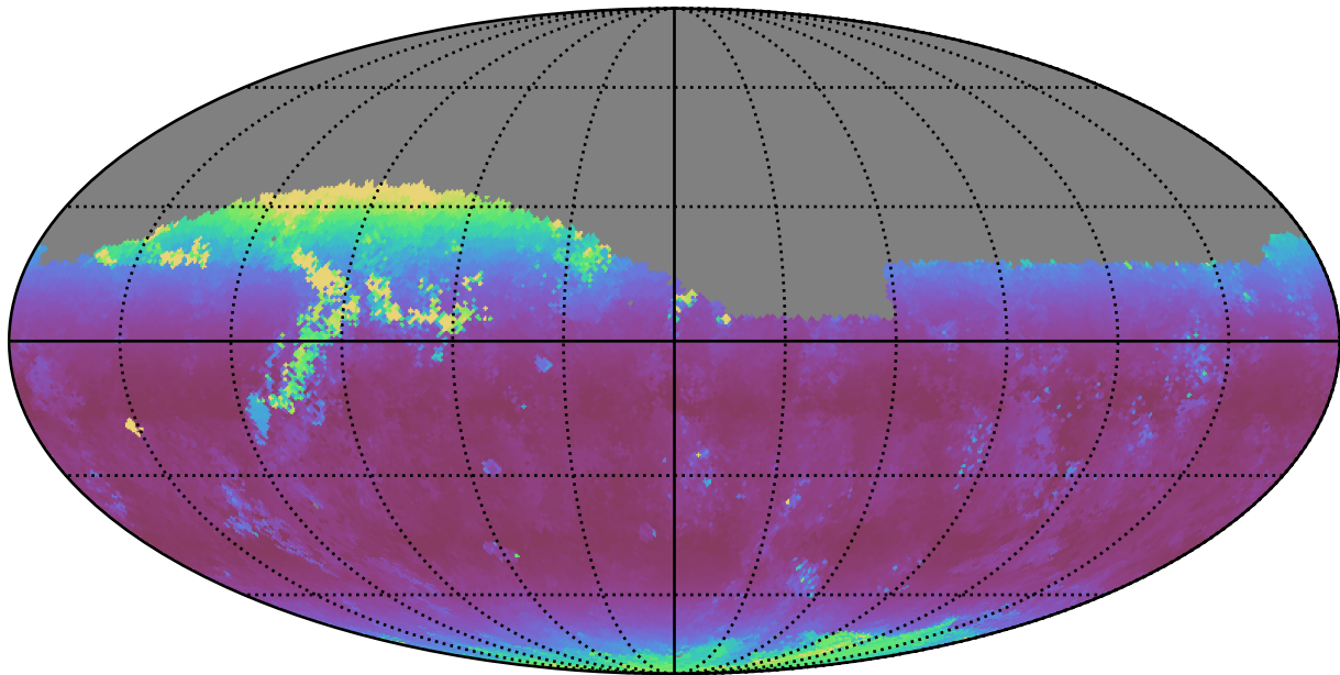
too_elab_r8_d2_griz_v3.4_10yrs Yr 1 z band: Median airmass
