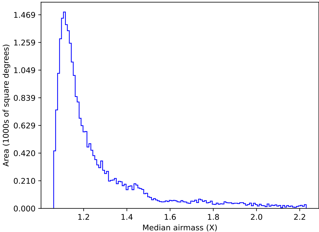
too_elab_r8_d2_griz_v3.4_10yrs Yr 1 z band: Median airmass
