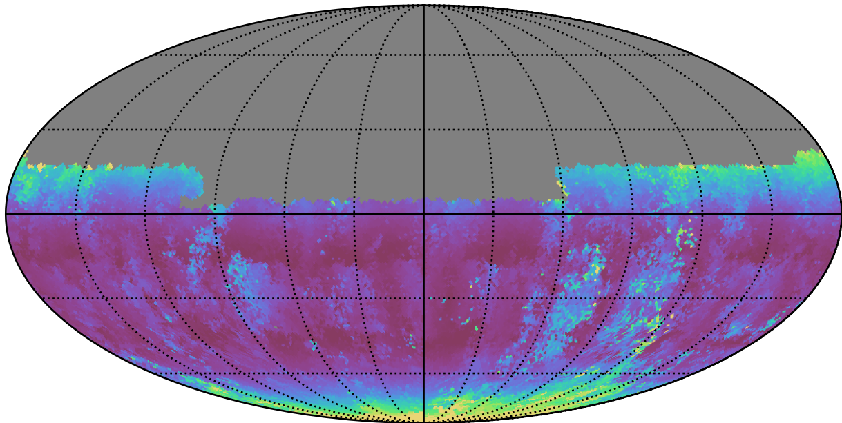
too_elab_r8_d2_griz_v3.4_10yrs Yr 1 u band: Median airmass
