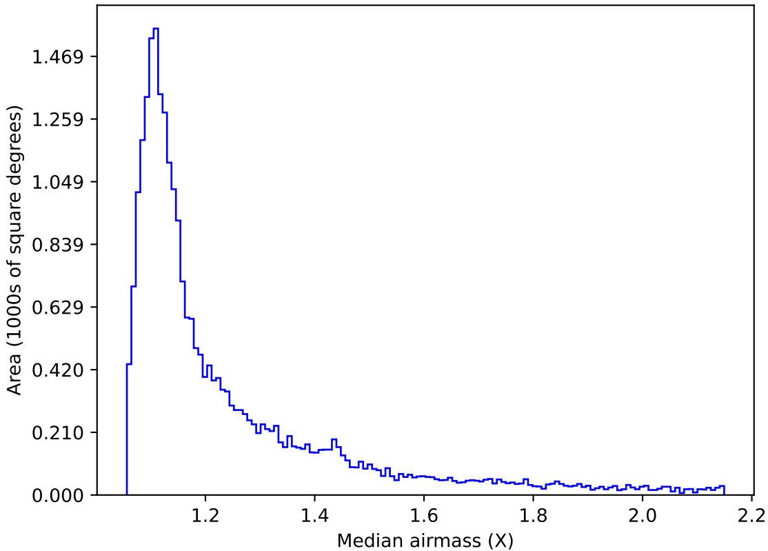
too_elab_r8_d2_griz_v3.4_10yrs Yr 1 r band: Median airmass
