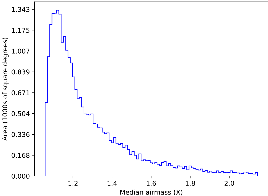
too_elab_r8_d2_griz_v3.4_10yrs Yr 1 g band: Median airmass
