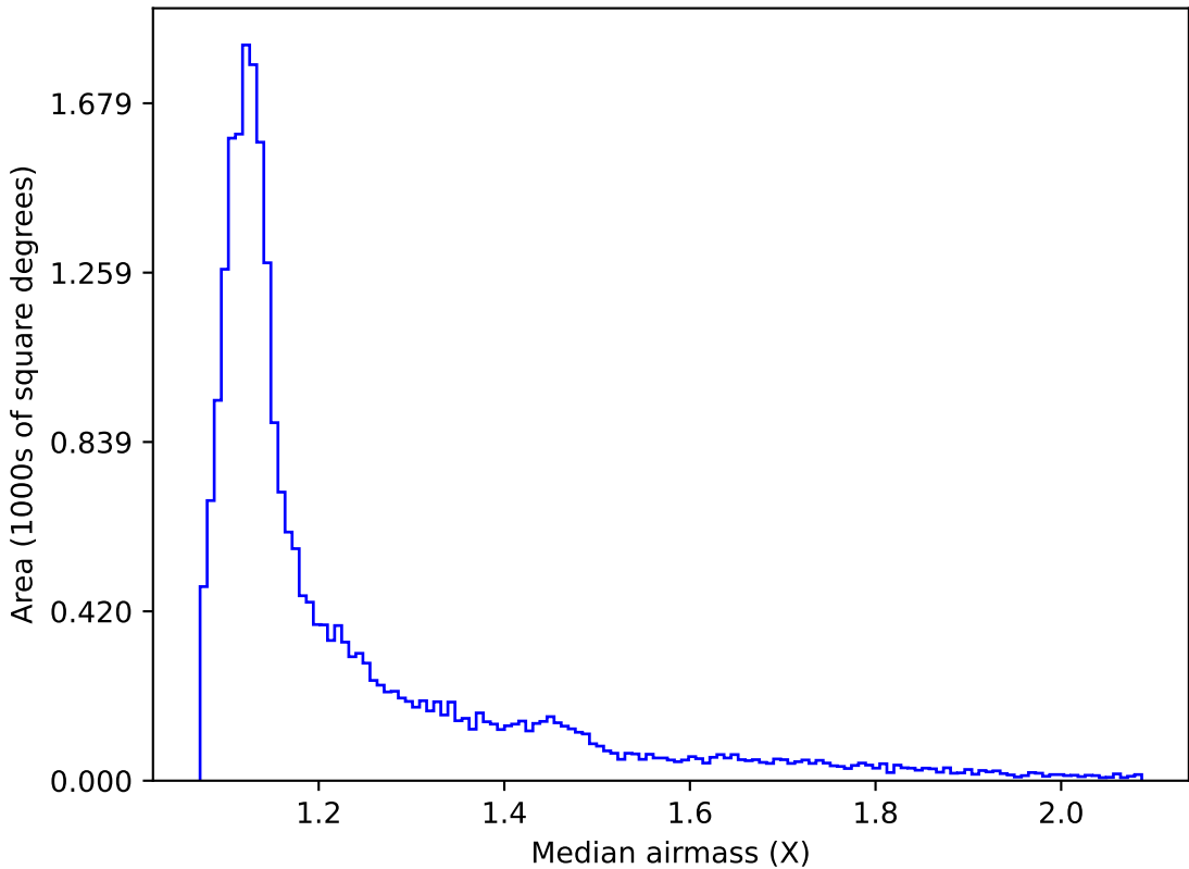
too_elab_r8_d2_griz_v3.4_10yrs Yr 1 all bands: Median airmass
