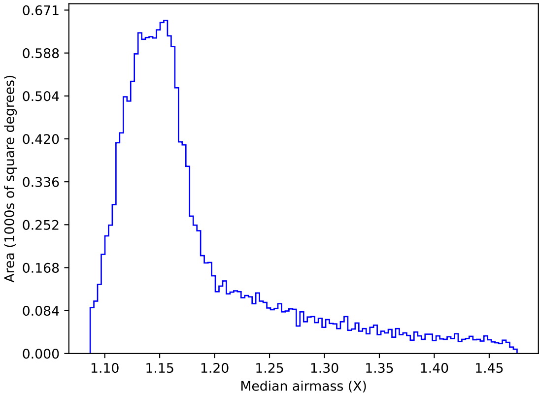
too_elab_r8_d2_griz_v3.4_10yrs WFD z band: Median airmass
