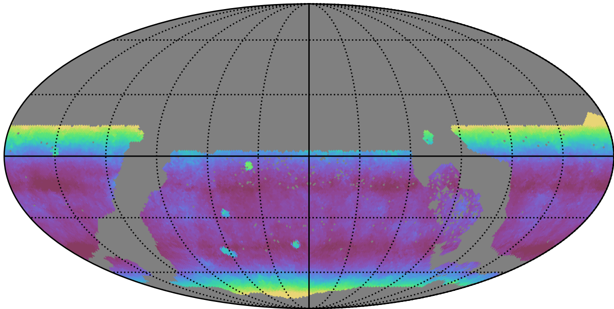
too_elab_r8_d2_griz_v3.4_10yrs WFD y band: Median airmass
