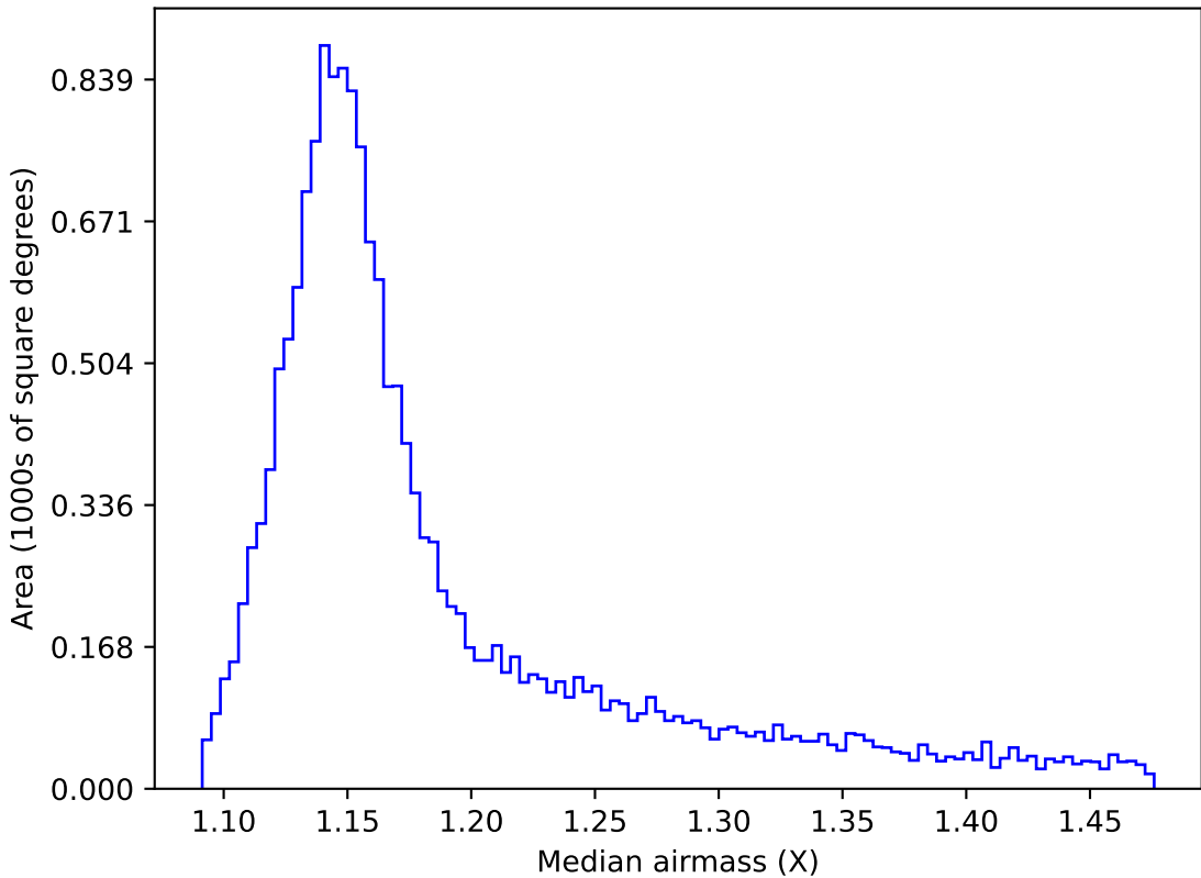
too_elab_r8_d2_griz_v3.4_10yrs WFD y band: Median airmass
