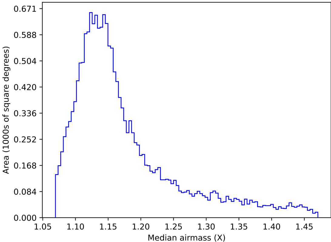
too_elab_r8_d2_griz_v3.4_10yrs WFD u band: Median airmass
