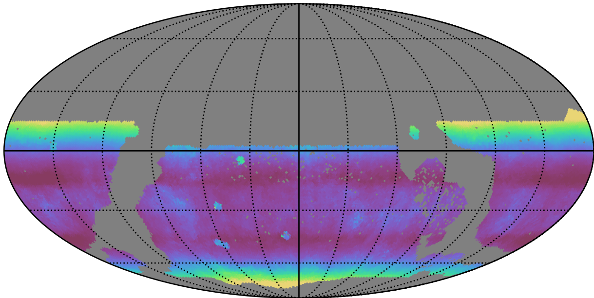
too_elab_r8_d2_griz_v3.4_10yrs WFD r band: Median airmass
