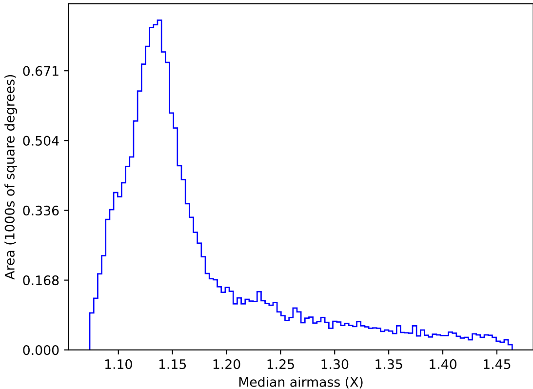
too_elab_r8_d2_griz_v3.4_10yrs WFD r band: Median airmass
