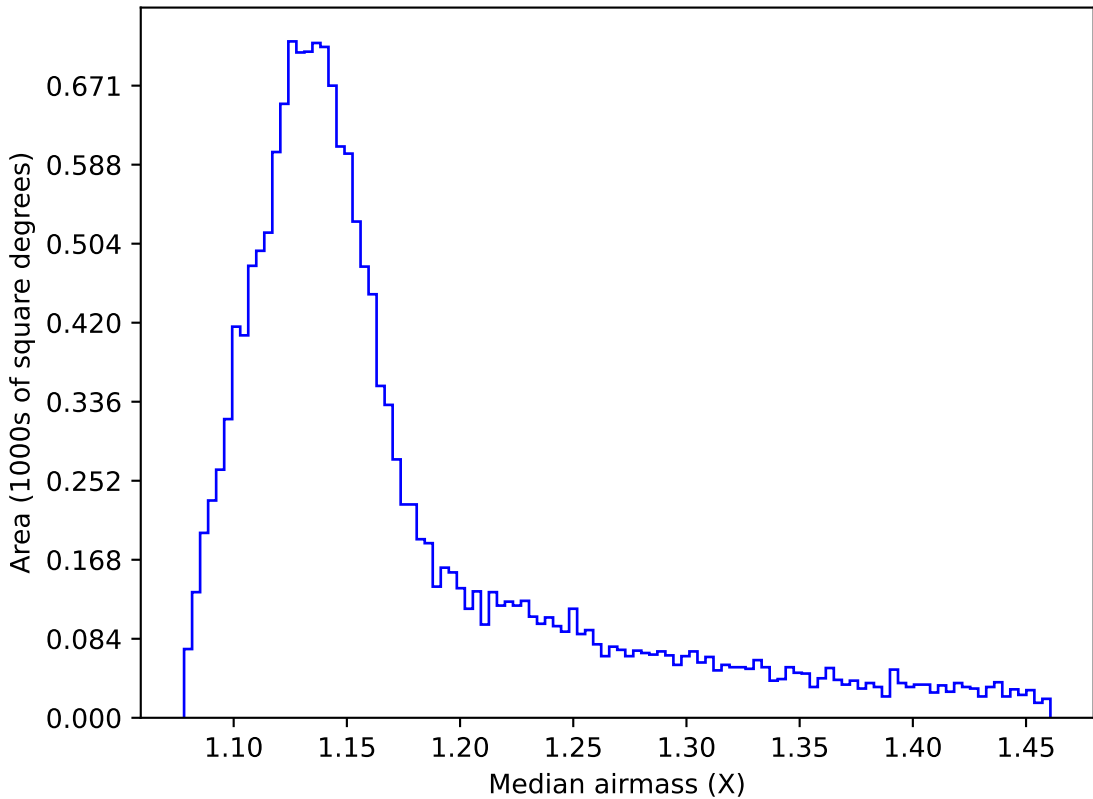
too_elab_r8_d2_griz_v3.4_10yrs WFD i band: Median airmass
