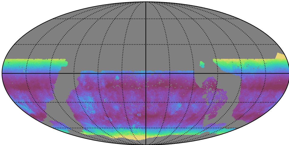
too_elab_r8_d2_griz_v3.4_10yrs WFD g band: Median airmass
