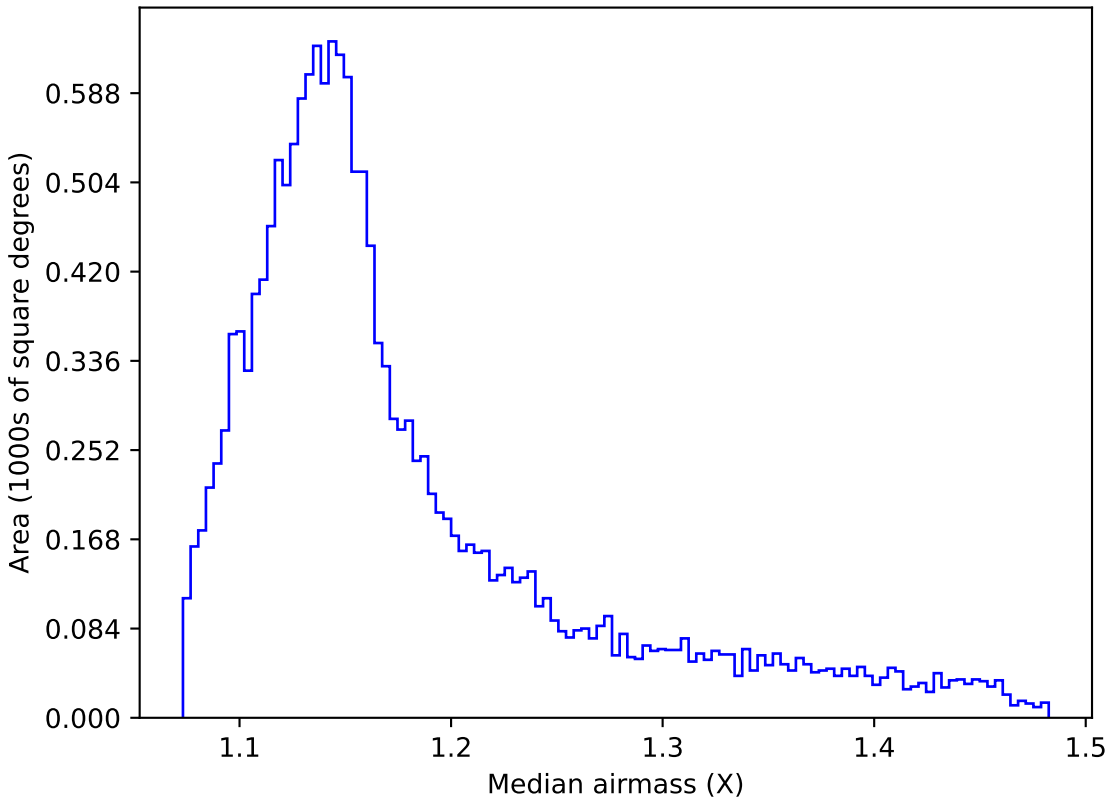
too_elab_r8_d2_griz_v3.4_10yrs WFD g band: Median airmass
