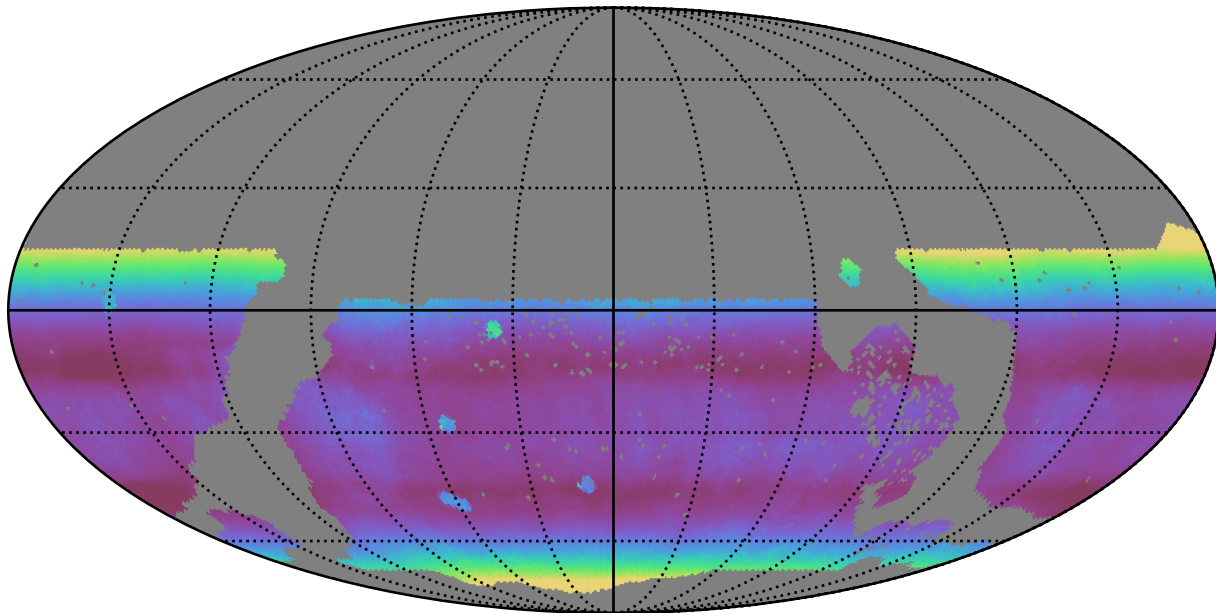
too_elab_r8_d2_griz_v3.4_10yrs WFD all bands: Median airmass
