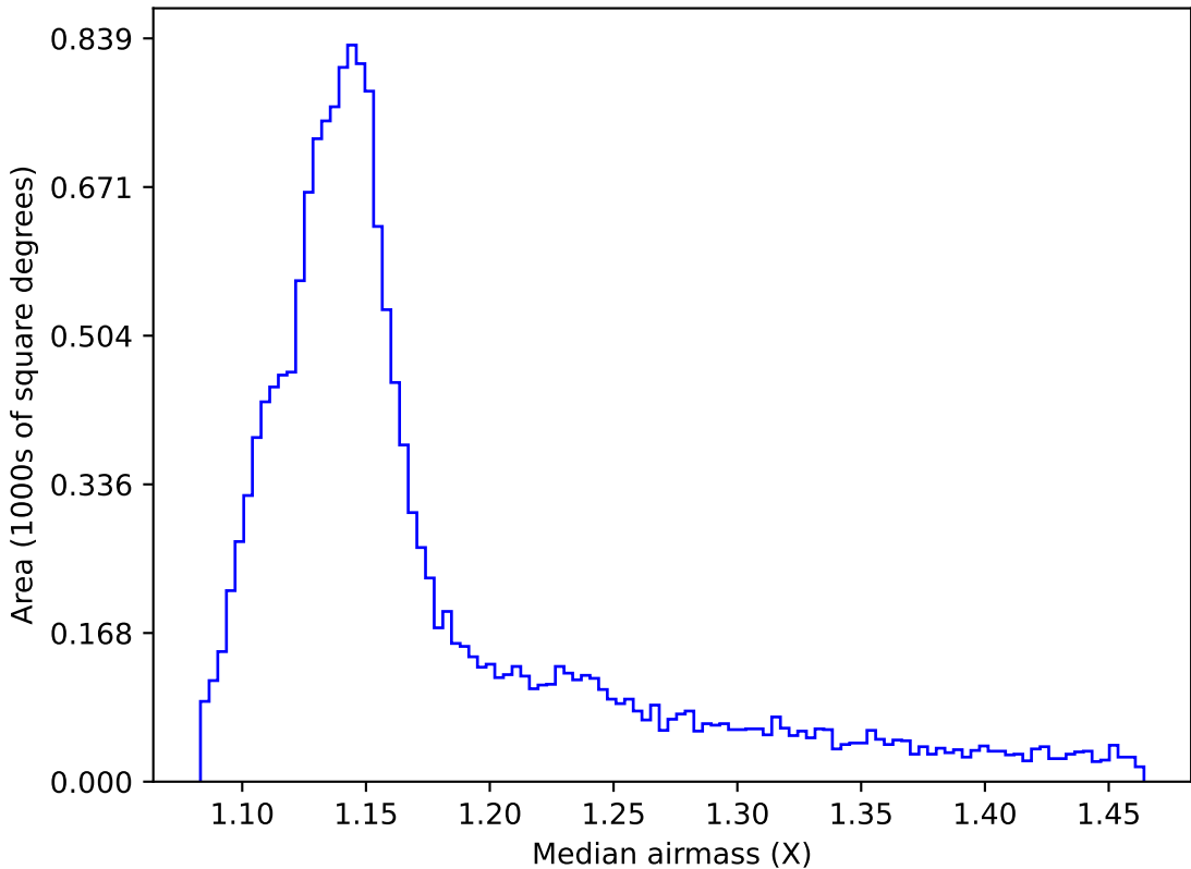
too_elab_r8_d2_griz_v3.4_10yrs WFD all bands: Median airmass
