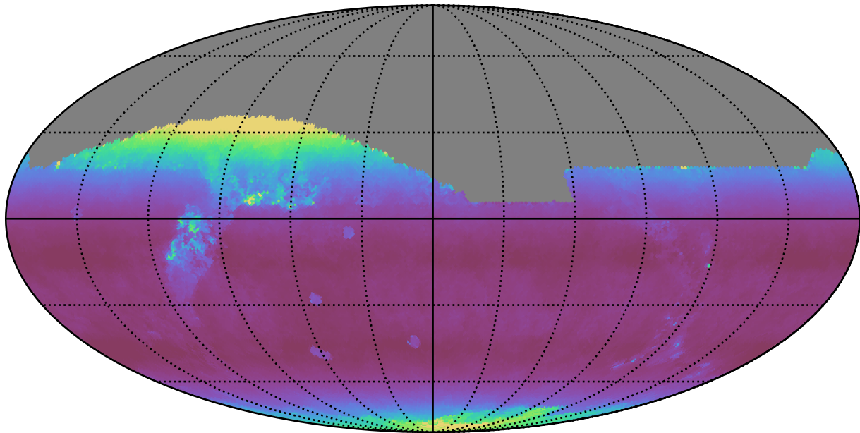
too_elab_r8_d2_griz_v3.4_10yrs All sky z band: Median airmass
