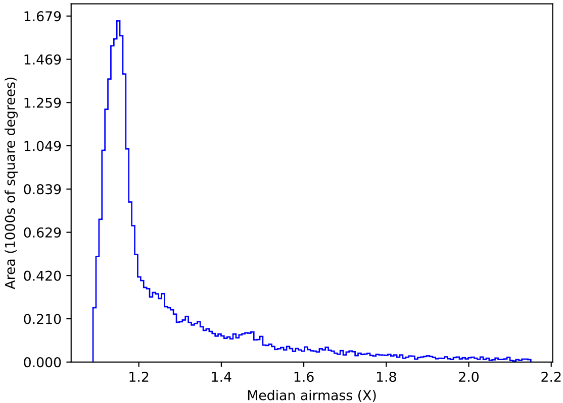
too_elab_r8_d2_griz_v3.4_10yrs All sky z band: Median airmass
