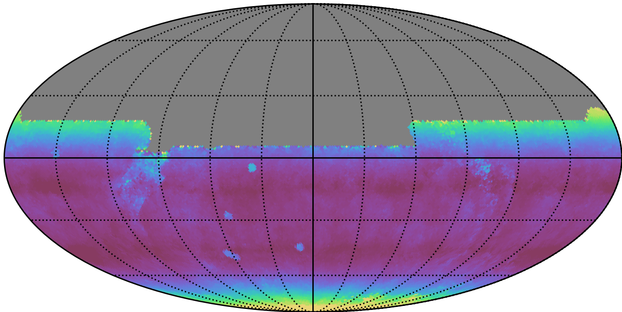
too_elab_r8_d2_griz_v3.4_10yrs All sky y band: Median airmass
