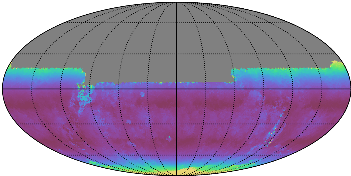
too_elab_r8_d2_griz_v3.4_10yrs All sky u band: Median airmass
