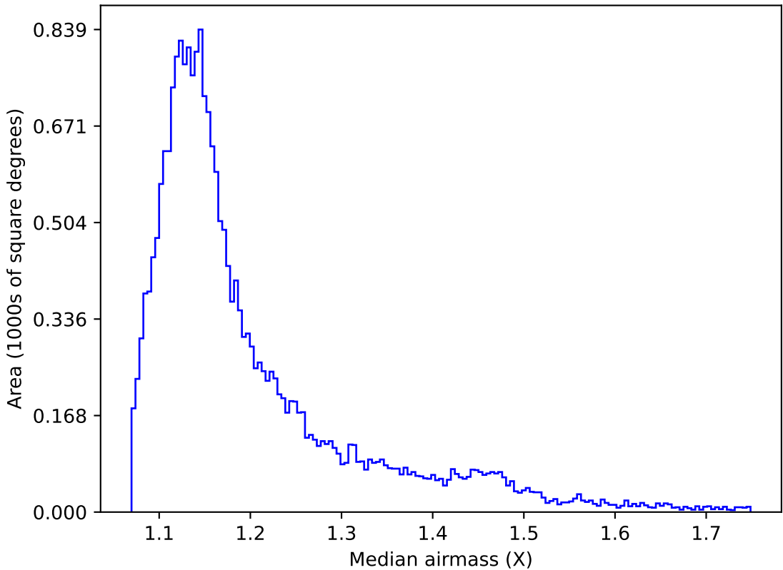
too_elab_r8_d2_griz_v3.4_10yrs All sky u band: Median airmass
