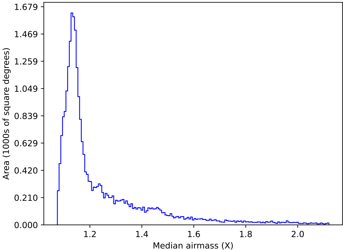
too_elab_r8_d2_griz_v3.4_10yrs All sky r band: Median airmass
